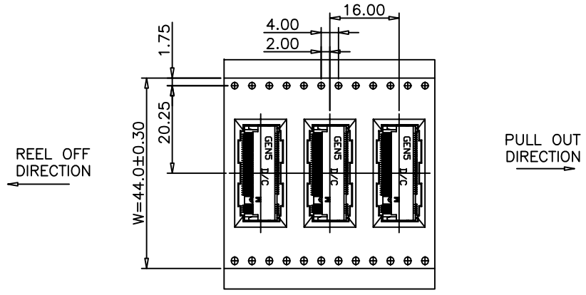
DETAIL X SCALE 3:1
