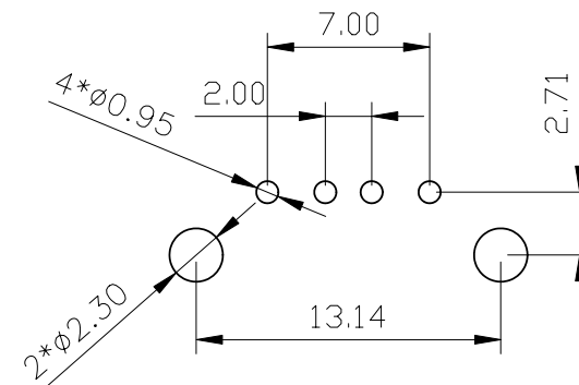
PCB LAYOUT (TOLERANCE: ±0.05mm)
