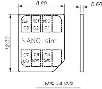
【 SIM Card Pin Assignments 】
