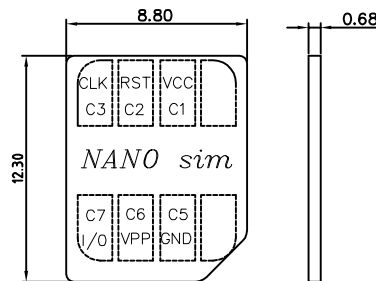
NANO SIM CARD
