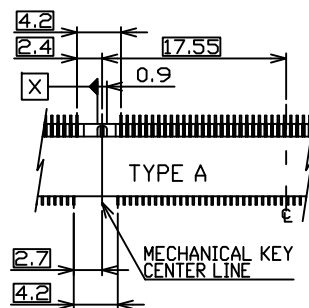
DETAIL E MECHANICAL KEY TYPE
