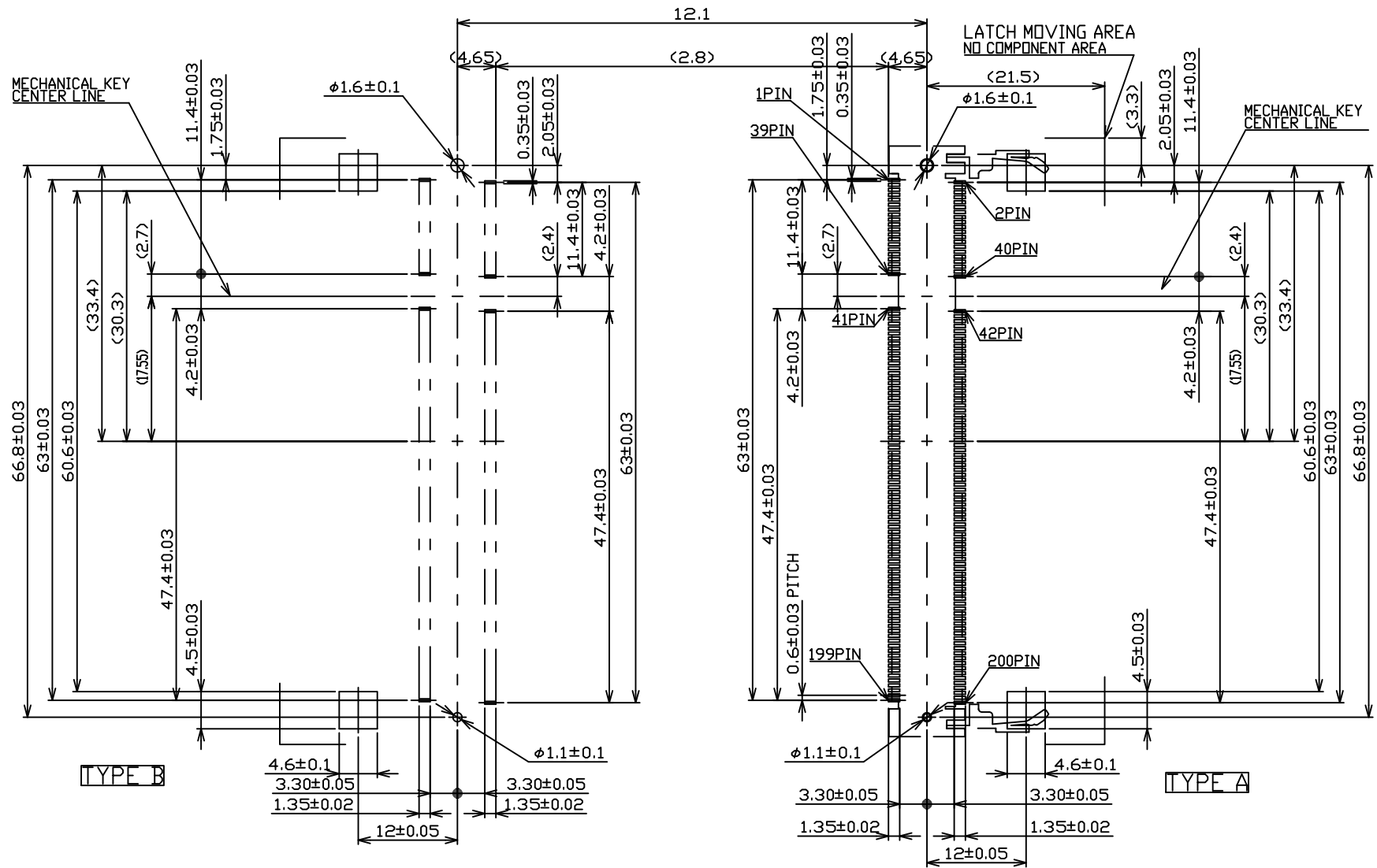
RECOMMENDED MOUNTING P.C. BOARD PATTERN LAYOUT DIM.
