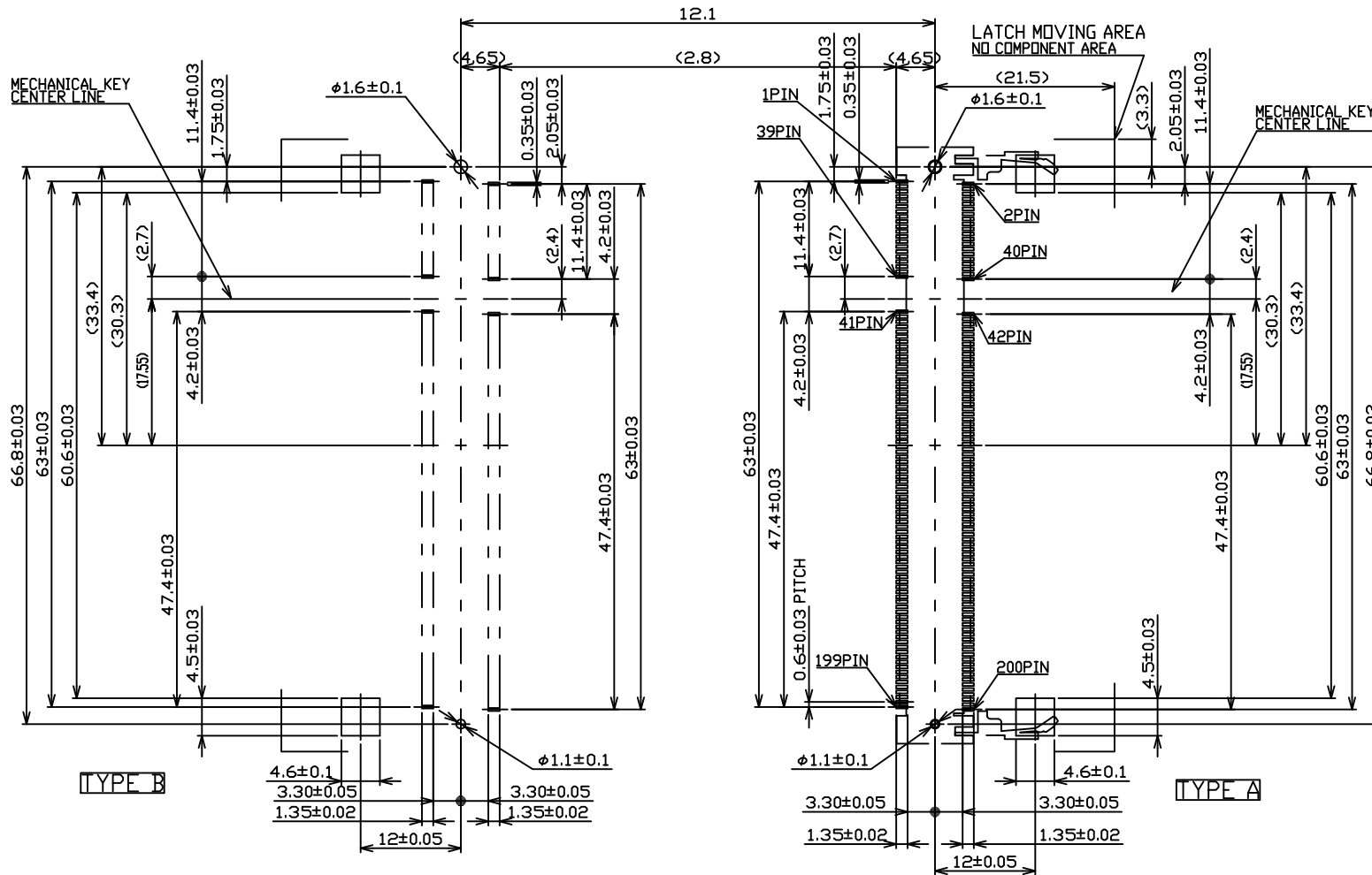
RECOMMENDED MOUNTING P.C. BOARD PATTERN LAYOUT DIM.
