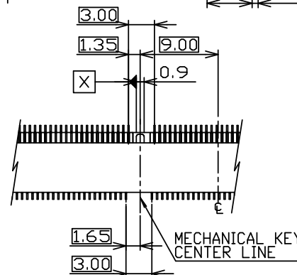
DETAIL E MECHANICAL KEY TYPE
